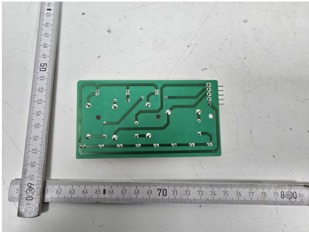
< Indicator PCB >
